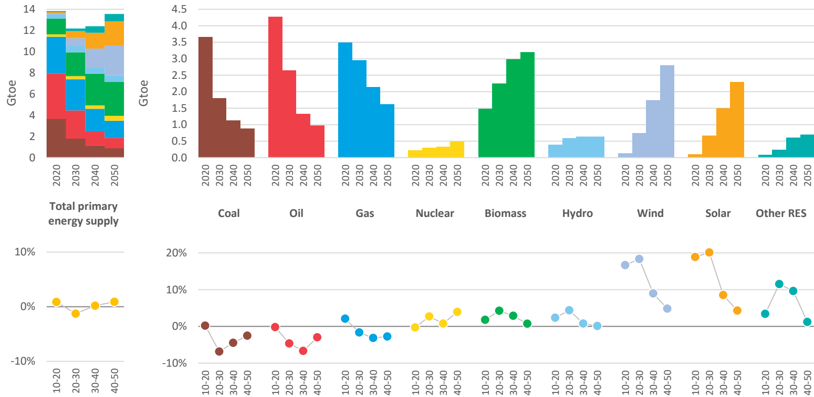
Figure 4: Global total primary energy supply by fuel, and decadal growth rates, 1.5°C scenario
