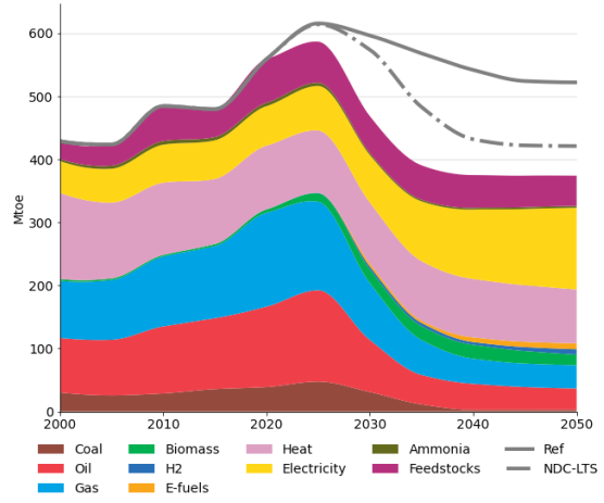
Final Energy consumption - 1.5C
