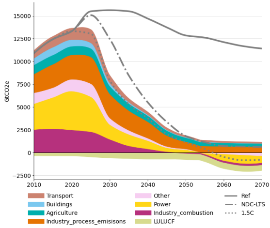
Emissions by scenario and sectoral breakdown of 1.5C scenario
