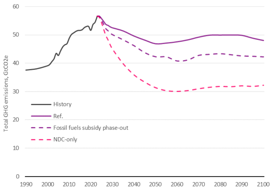
Figure 11: Global GHG emissions, by scenario
