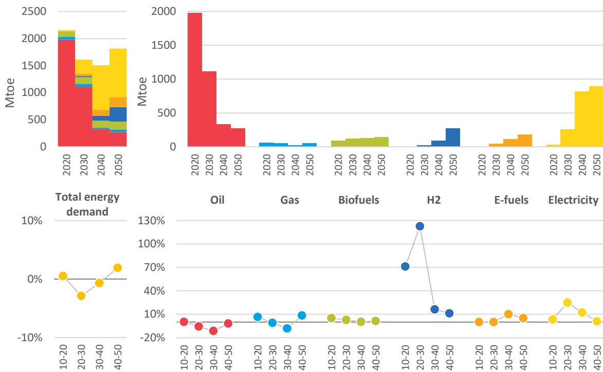
Figure 7: Global transport energy demand by fuel, and decadal growth rates, 1.5°C scenario
