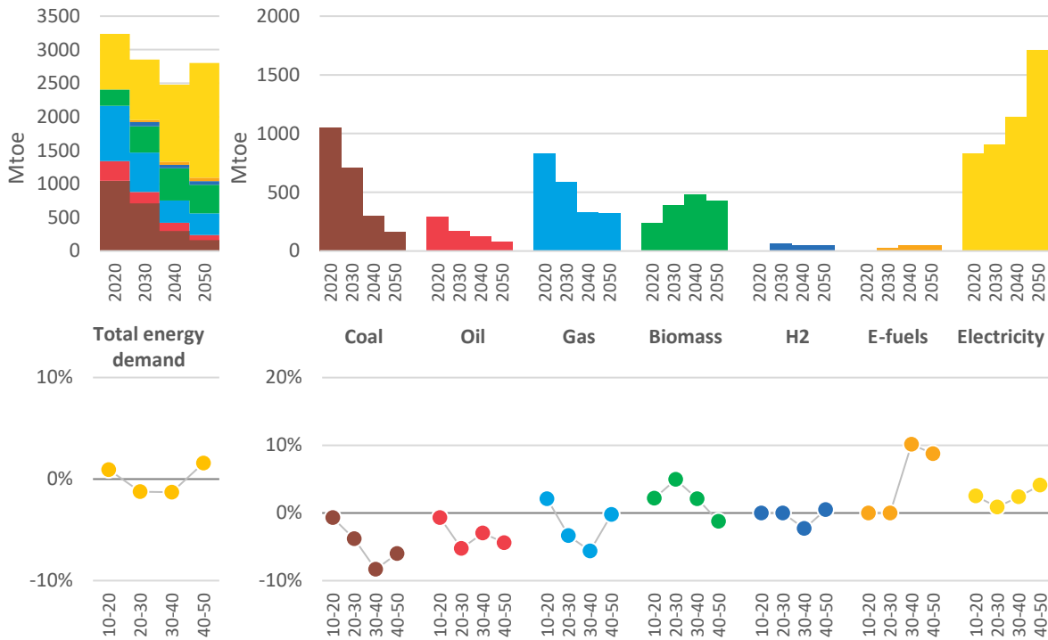
Figure 6: Global industry energy demand by fuel, and decadal growth rates, 1.5°C scenario
