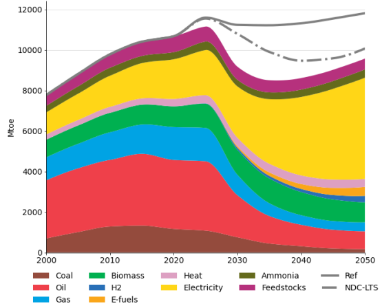
Final Energy consumption - 1.5C
