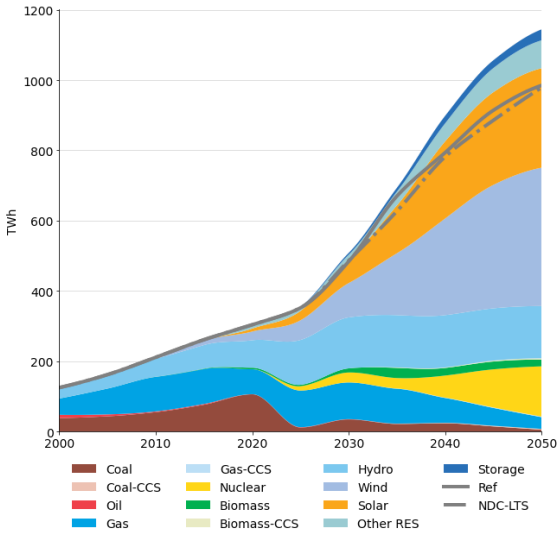
Power Generation - 1.5C
