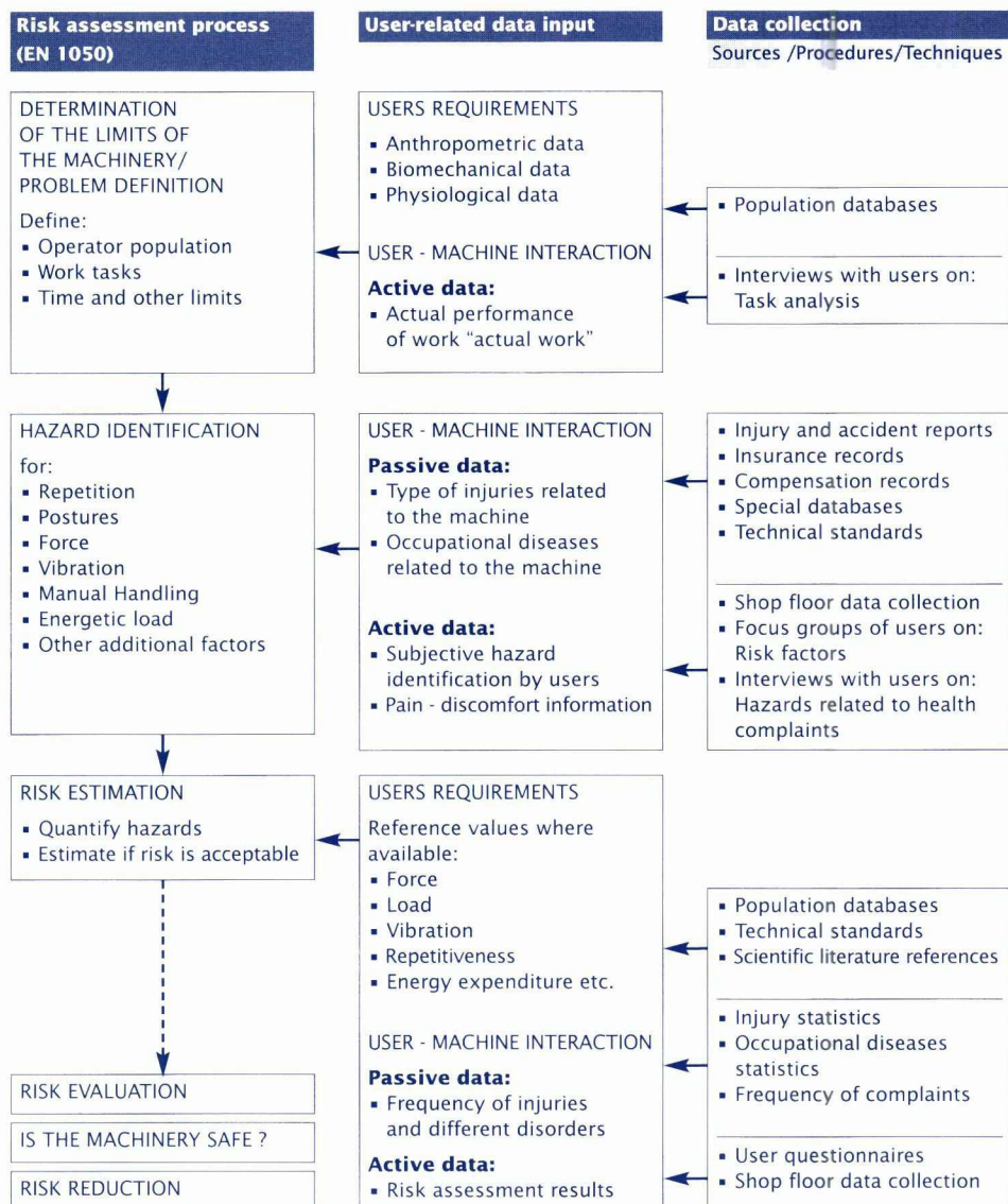
DIAGRAM: Risk estimation process for MSD risk factors on machinery design - users' input
